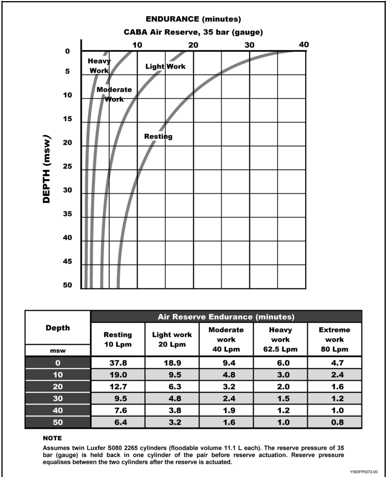
Figure 4-2 CABA Reserve with CABA Endurance Chart
