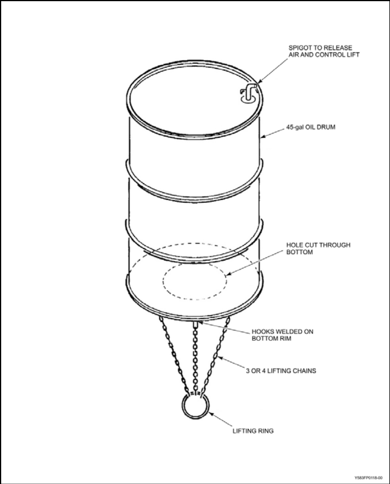
Figure 5-22 Improvised Lifting Aid Using an Oil Drum
