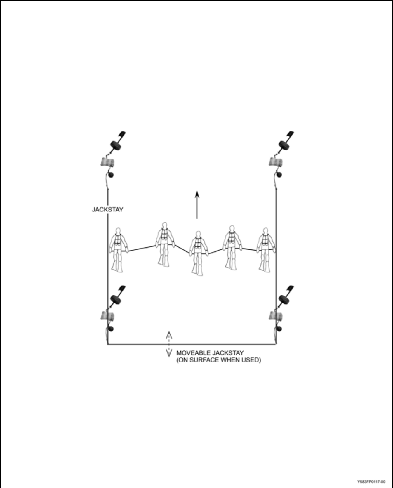
Figure 5-21 Multiple Diver Seabed Search
