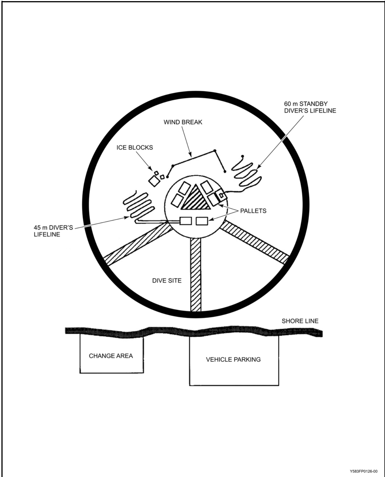
Figure 5B-3 Dive Set-up, Ice Diving
