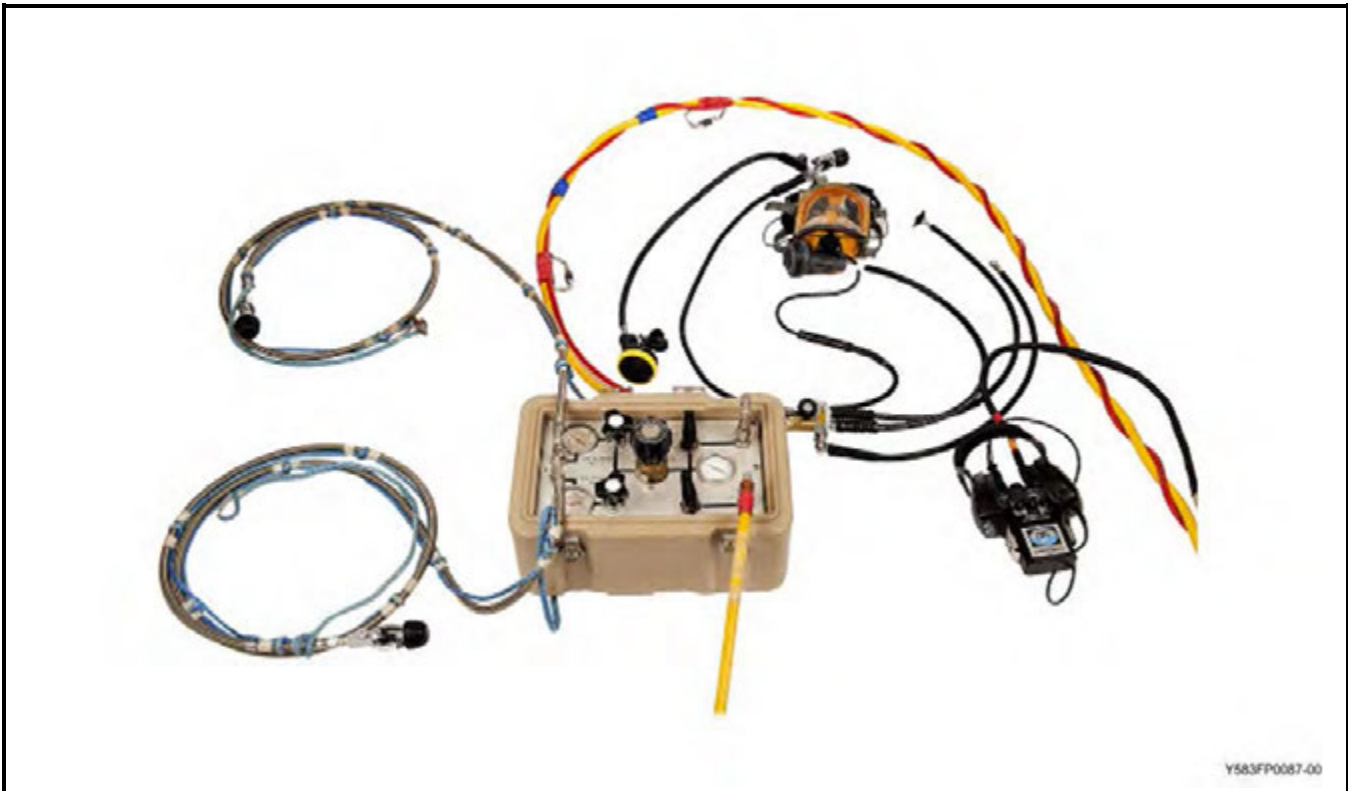
Figure 4-19 SBA, HP and IP Hose Whips – Redundant Second Stage
