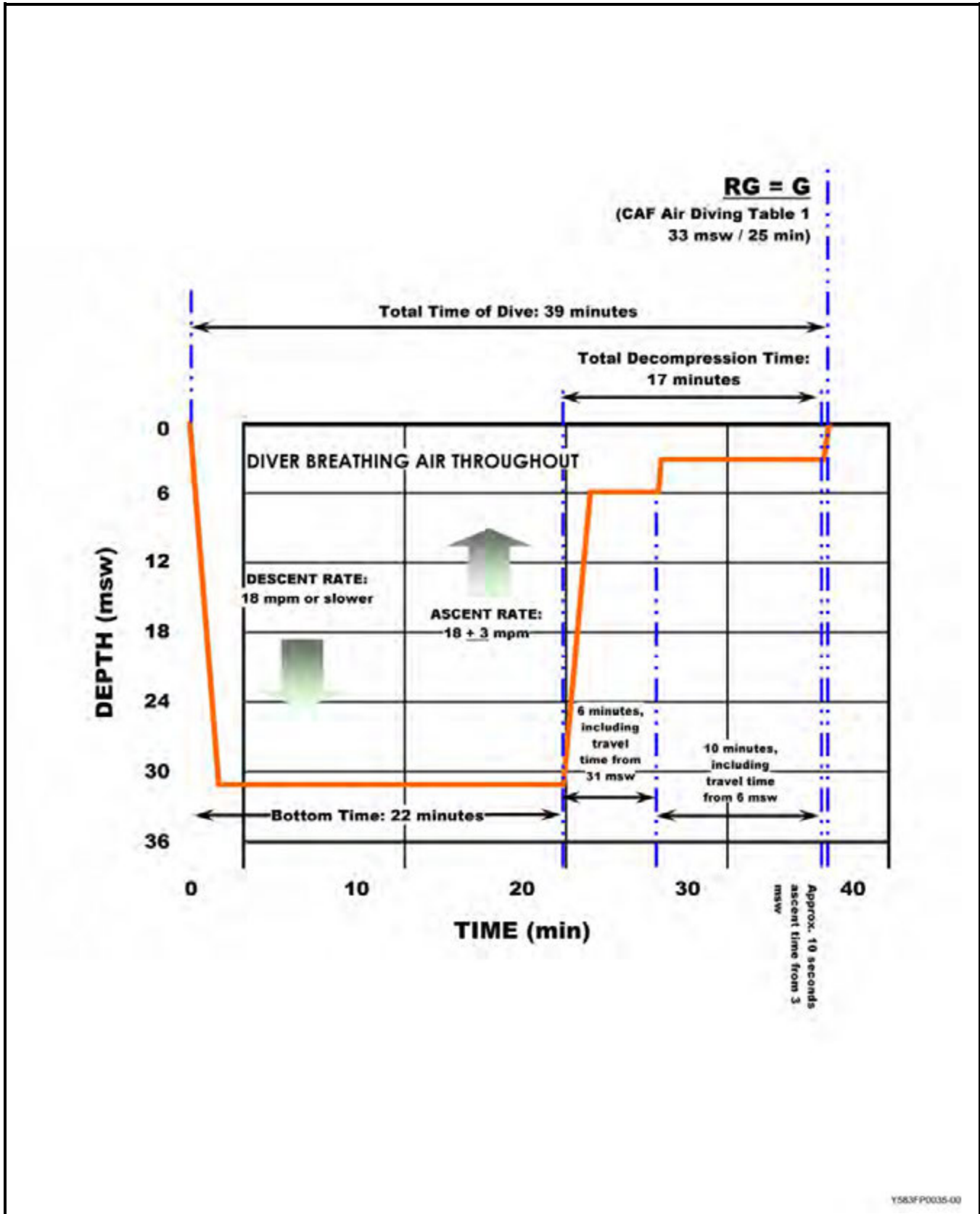
Figure 3-2 Standard Air Decompression Dive Profile, 31 msw/22 min (ref. Article 308, paragraph 8, Example 1 )
