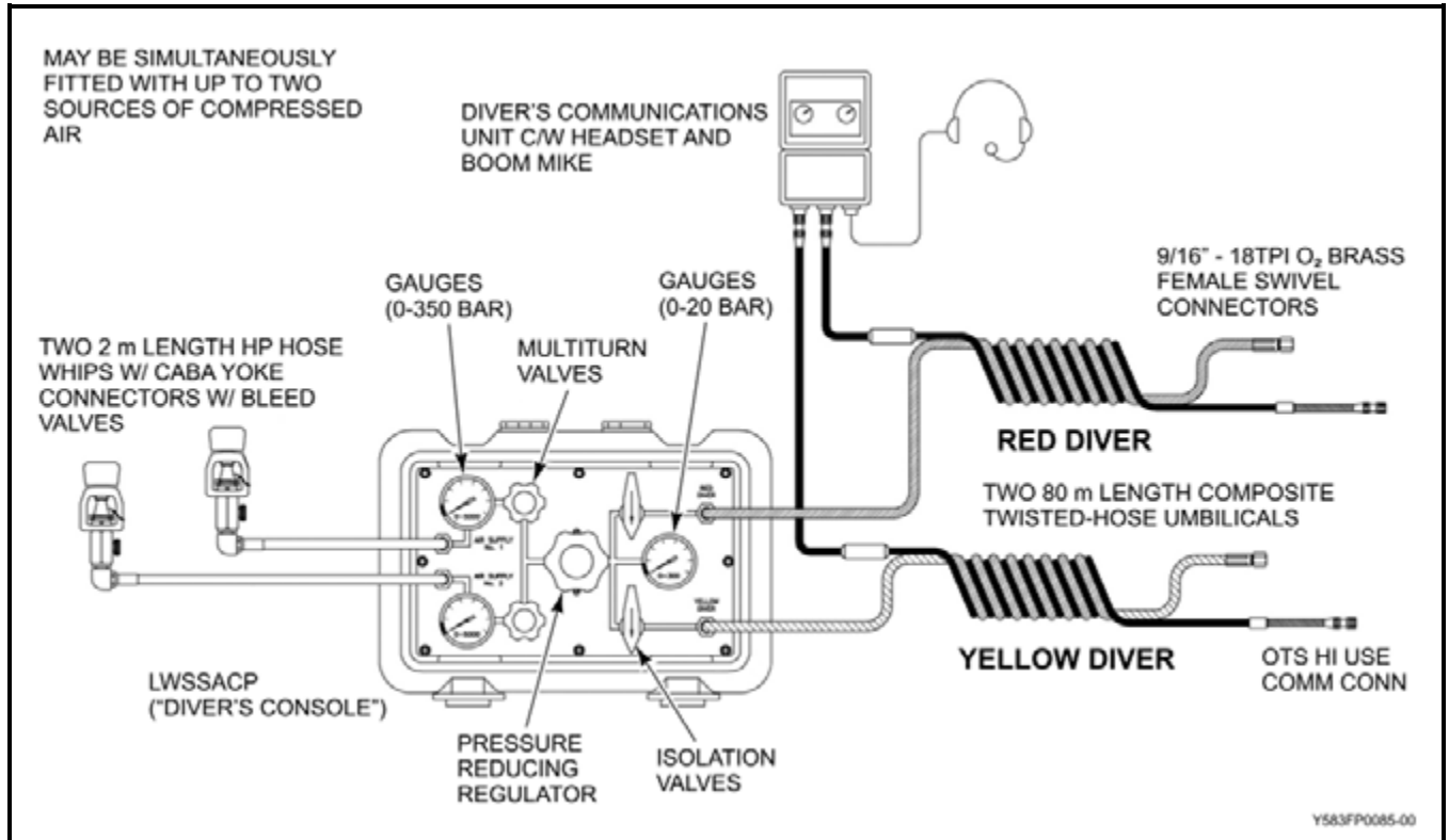
Figure 4-17 LWSSDE Console, Yokes and HP Hose Whips, Comms and Umbilicals
