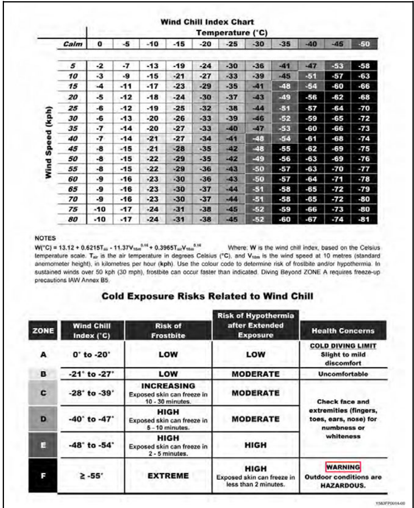
Figure 1-9 Wind Chill Index Chart
