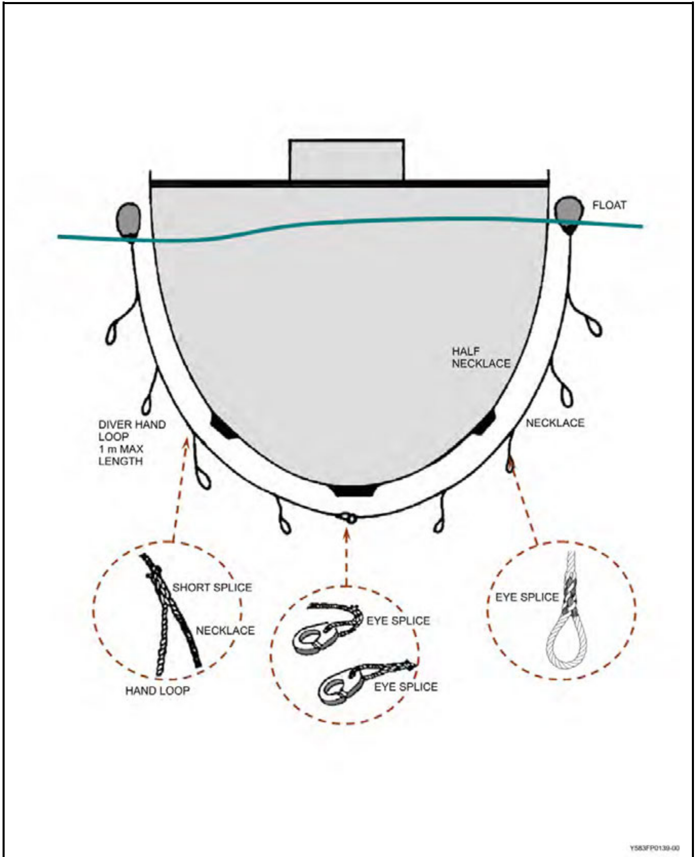
Figure 6-4 Search Scheme "A" – Necklace Search
