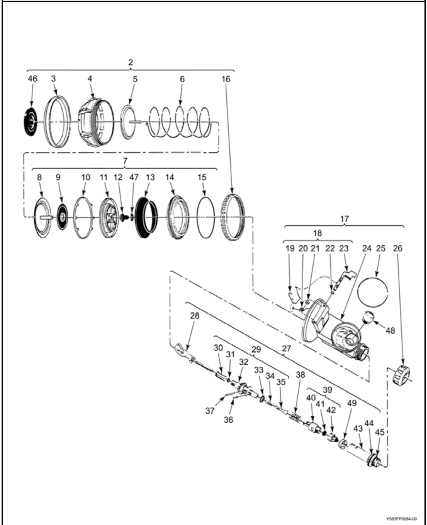
Figure 4-16 AGA MK II FFM Exhalation Assembly
