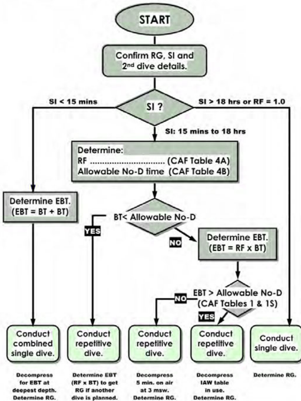
Figure 3-6 CAF Air Diving Tables Repetitive Diving Flowchart
