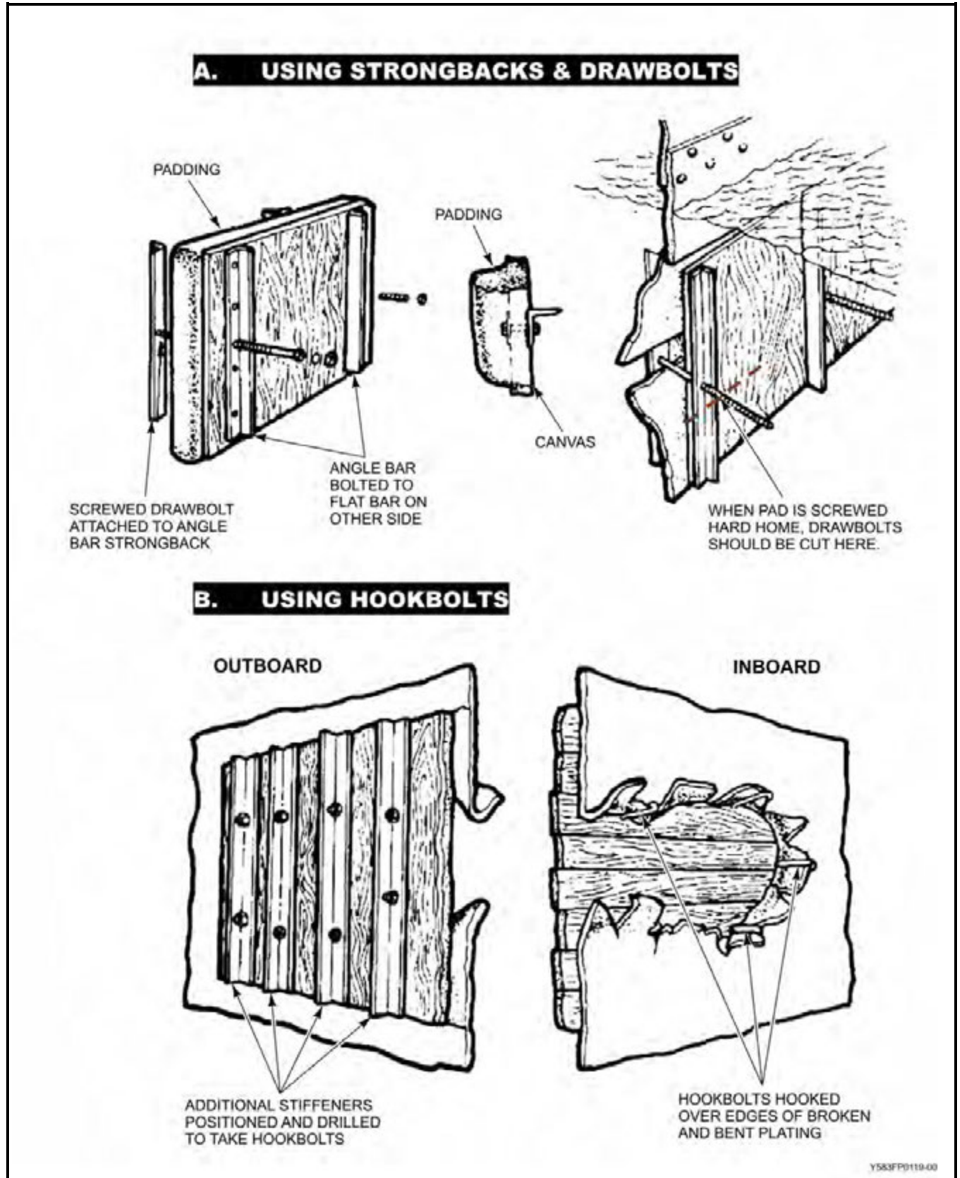
Figure 5-23 Methods of Securing a Timber Patch
