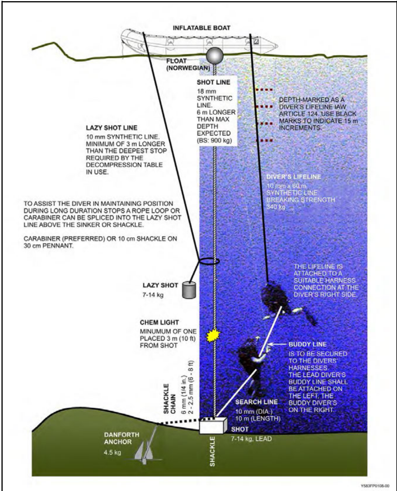
Figure 5-12 CABA Lazy Shot Diving, General Arrangement
