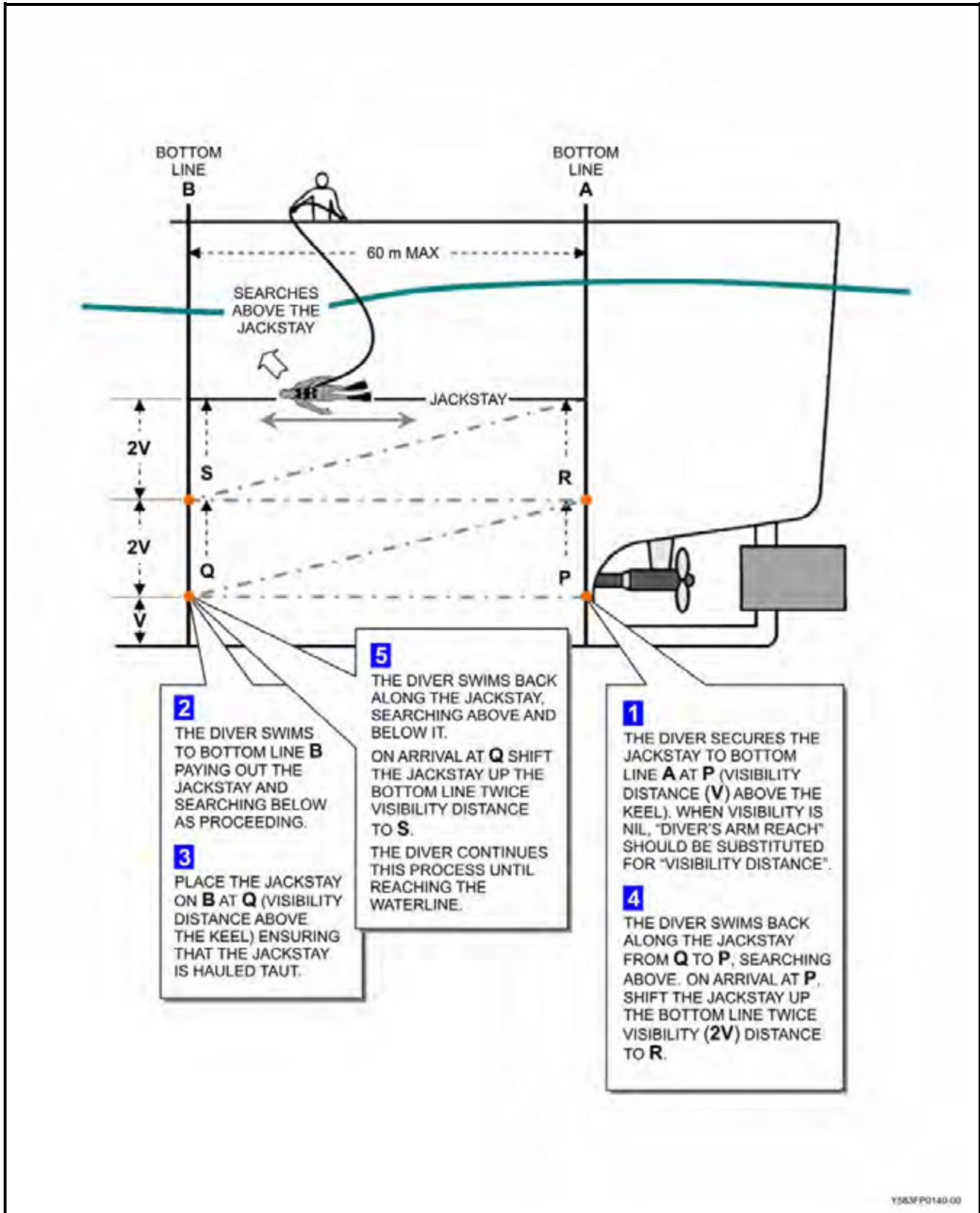
Figure 6-5 Search Scheme "B" – Zig-zag Search
