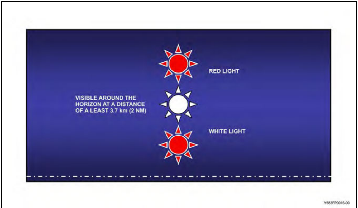
Figure 1-11 Diving Warning Signals (Small Craft, NIGHT)
