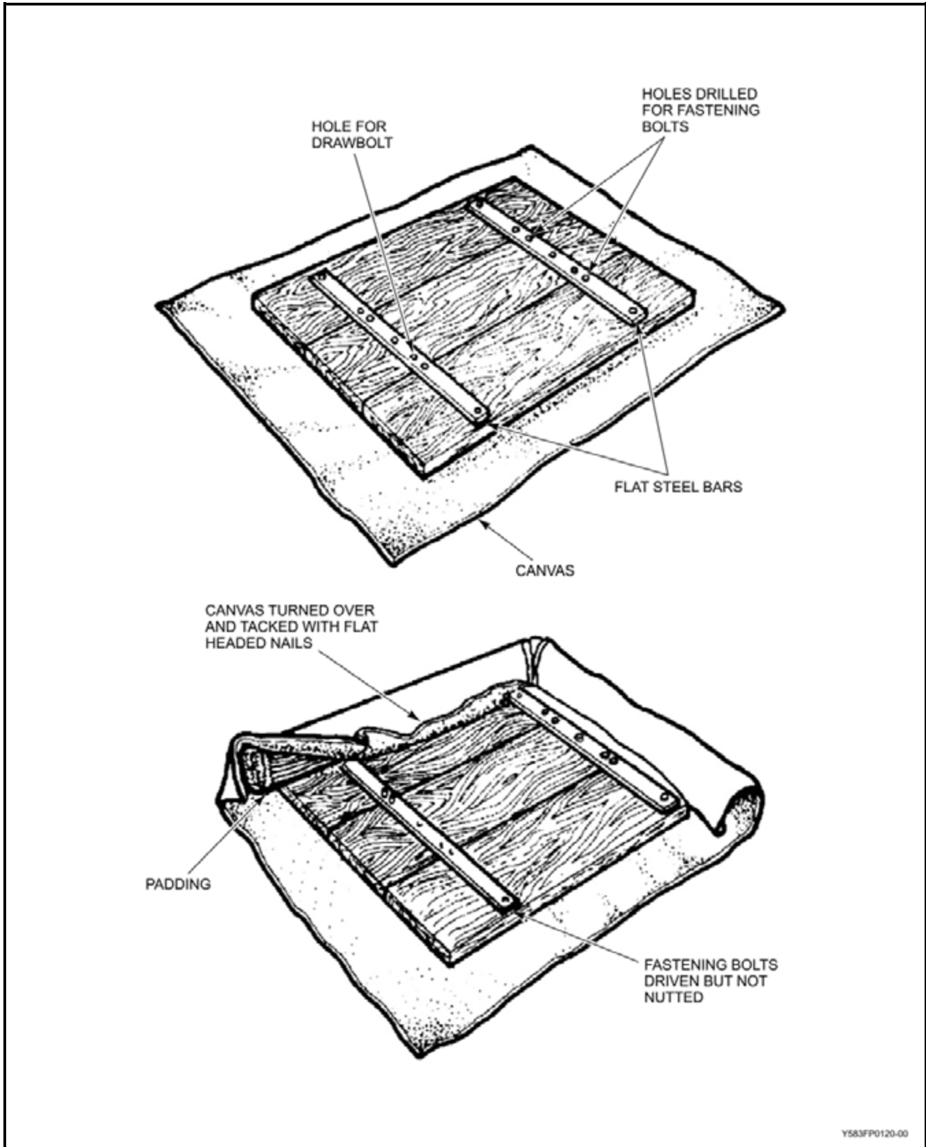
Figure 5-24 Timber Patch
