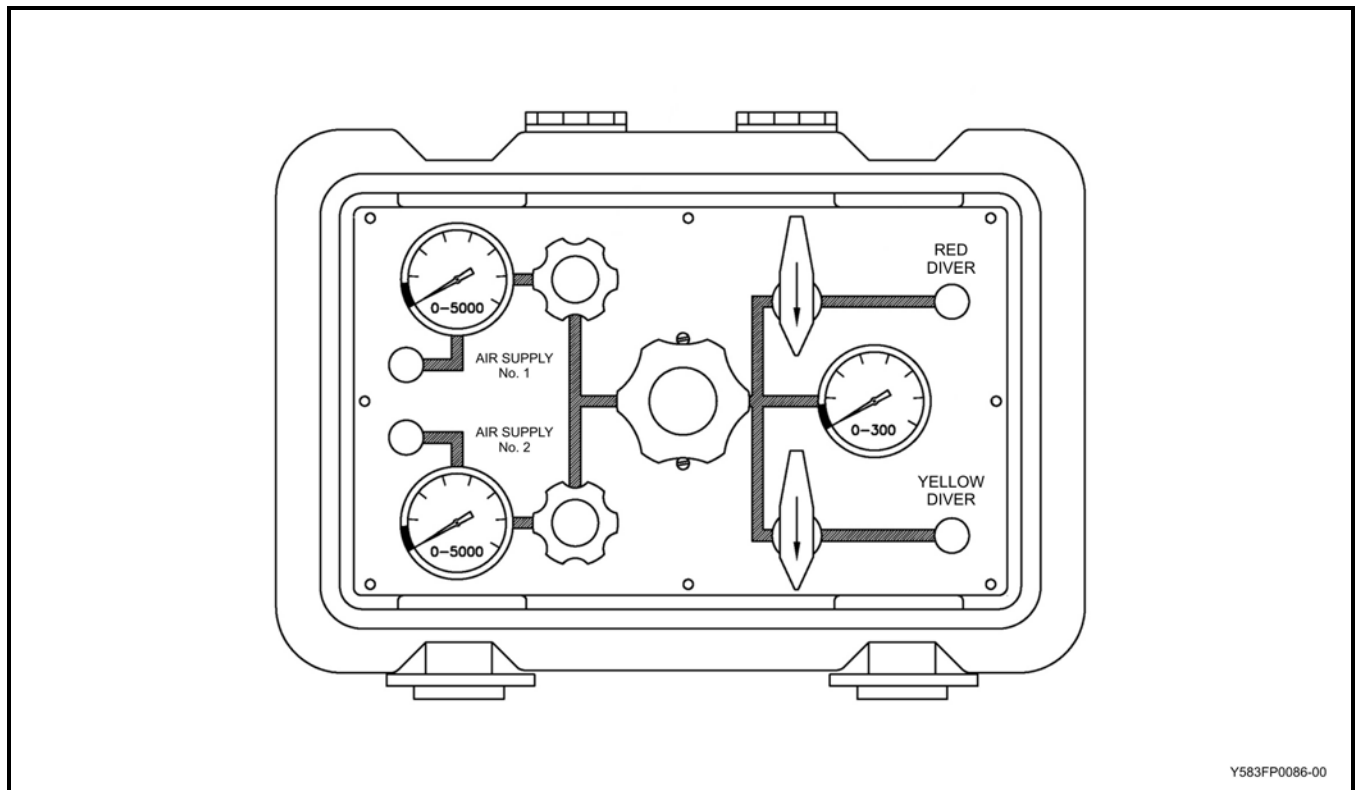
Figure 4-18 LWSSACP (Diver's Console)
