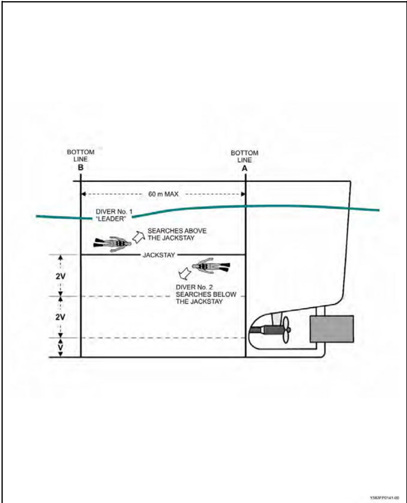
Figure 6-6 Search Scheme "C" – Ladder Search
