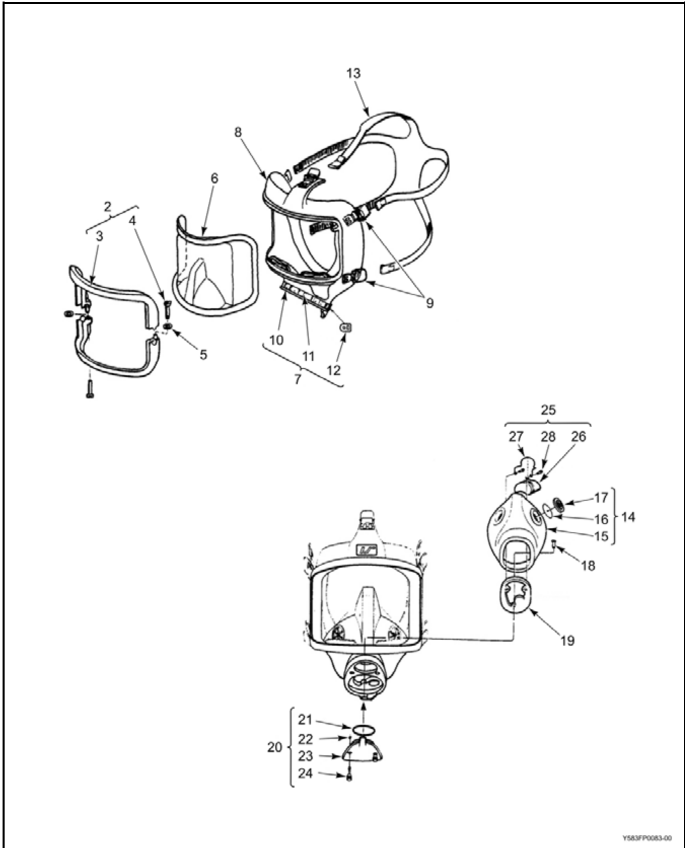
Figure 4-15 AGA MK II FFM Disassembly
